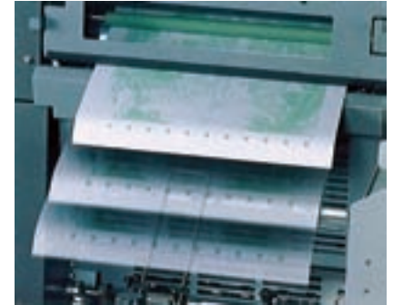
Professional features such as the computerized Ink Control System (ICS) and the semi-automatic plate changing help efficiently manage the increasing amount of multi-color work.
